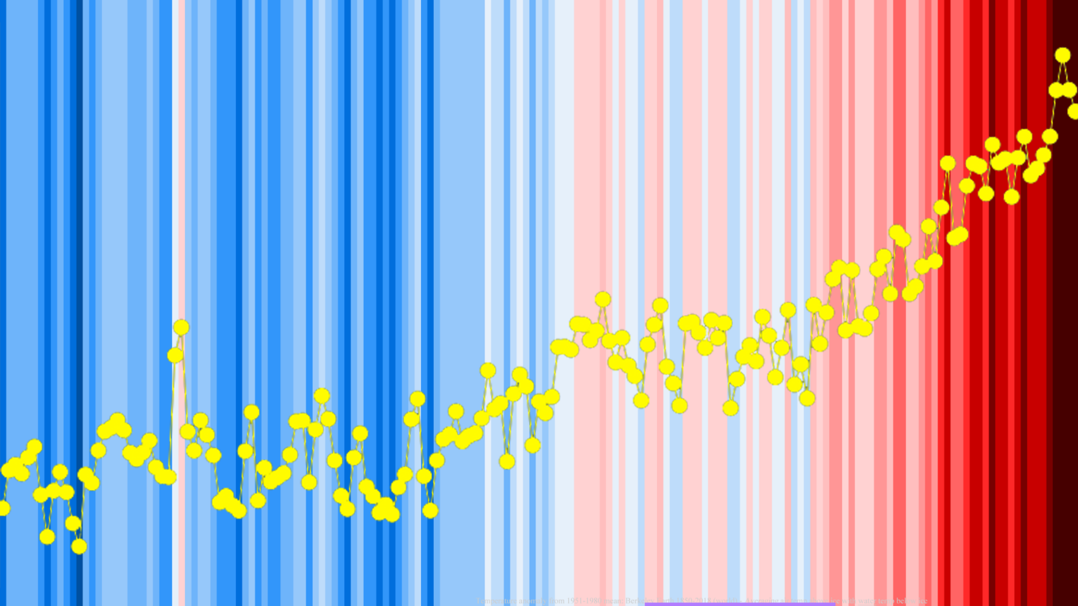
Temperature anomaly from 1951-1980 mean; Berkeley Earth 1850-2015 (excluding non-homogenized data with water temp below ice)
