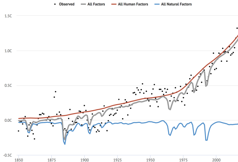
Global temperatures: Human and natural factors, 1850-2017
